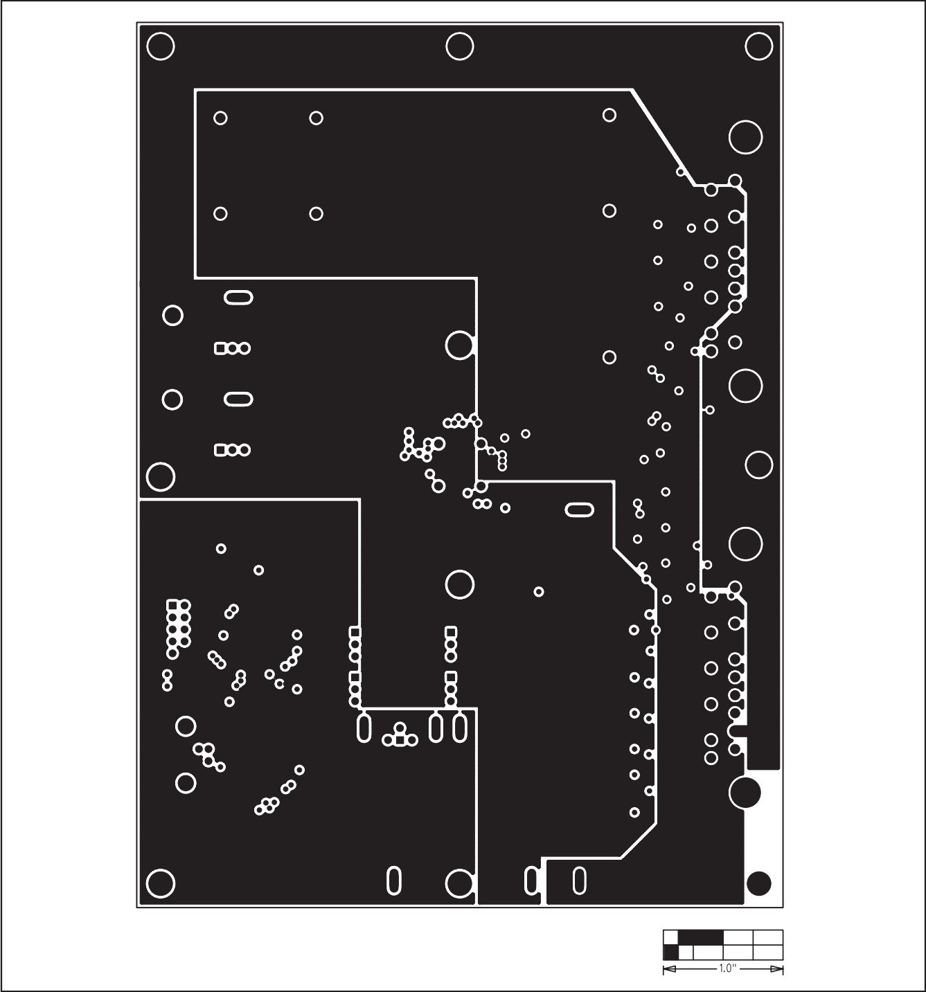
Figure 8. MAX9670 EV Kit PCB Layout—Inner Layer 2
